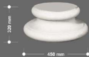
BB-C 300B Width: Ø450mm * Height: 320mm
